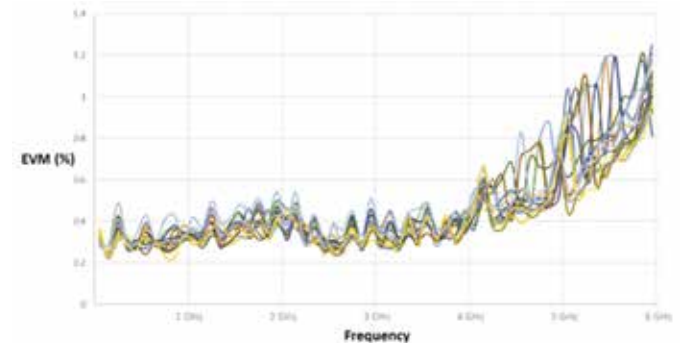
The VSG60A's EVM is specified and tested on each VSG. Shown are EVM test results for 17 VSGs.
