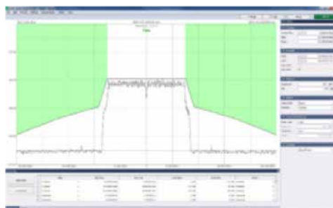
Spectrum Emission Mask Measurements
